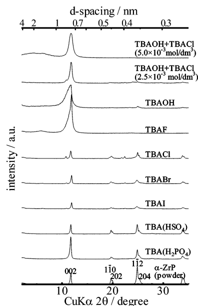
Figure 3. XRD patterns of \alpha -zirconium phosphate films electrochemically deposited from acetonitrile solution after reaction with neutral and basic TBA salts. \alpha -ZrP concentration = 6.7 \times 10^{-3} mol/dm 3 ; solvent = acetonitrile; deposition time = 15 min.
